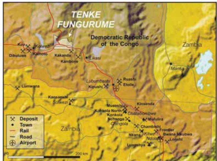
Location map of the Tenke-Fungurume mining district.
